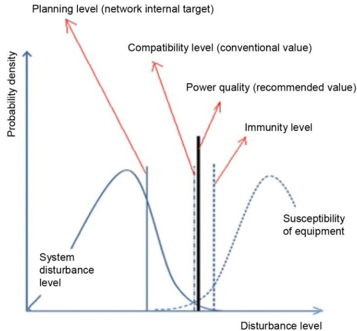
Figure F.2 – Relation between disturbance levels (schematic significance only)
